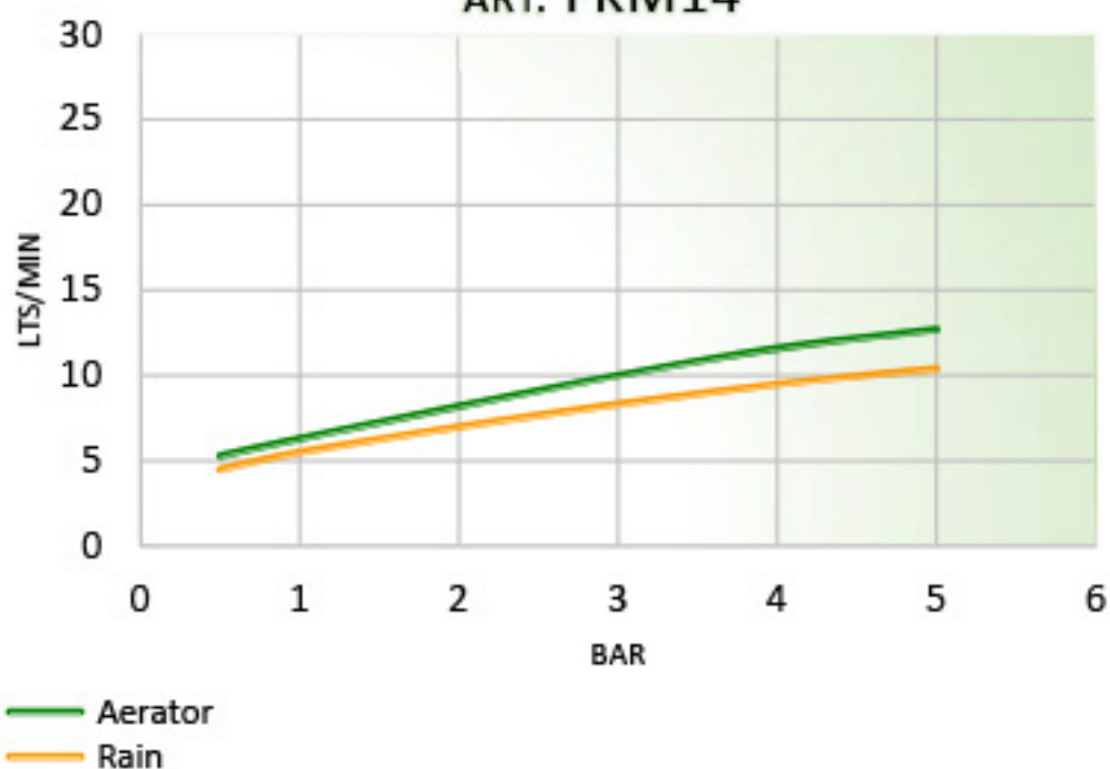
FLOW CHART ART. FKM14
