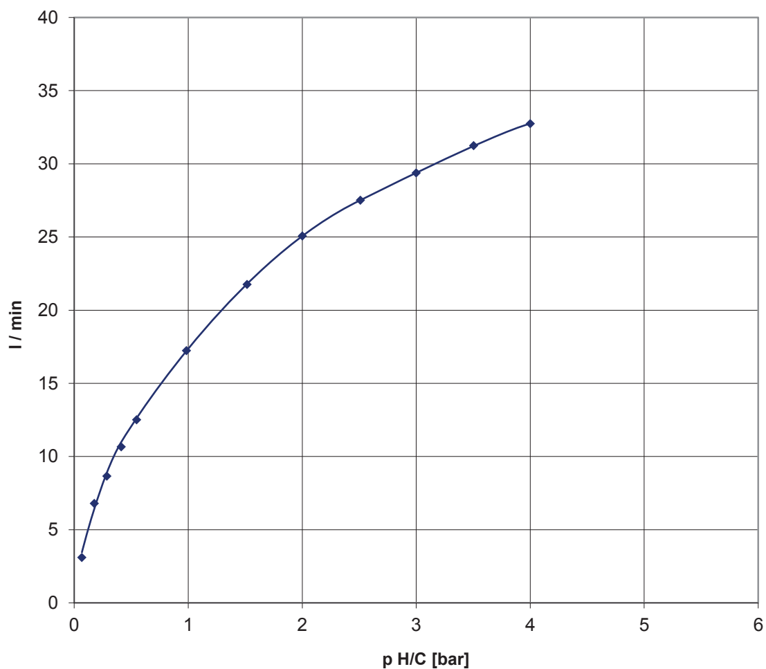
Flow rate
